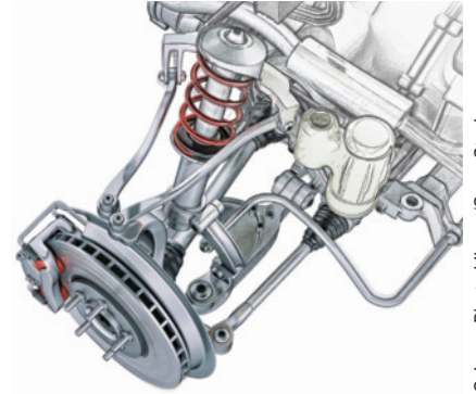
As in the case of the chapter-opening photograph, the spring and damper are coaxial in this multi-link automobile suspension.
