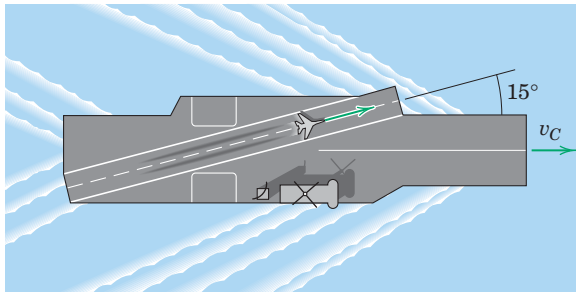
2/239 The launching catapult of the aircraft carrier gives the jet fighter a constant acceleration of 50 \text{ m/s}^2 from rest relative to the flight deck and launches the aircraft in a distance of 100 m measured along the angled takeoff ramp. If the carrier is moving at a steady 30 knots (1 knot = 1.852 km/h), determine the magnitude v of the actual velocity of the fighter when it is launched.
